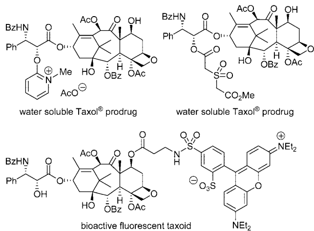
FIGURE 23. Molecular structures of selected designed analogs synthesized and biologically evaluated during the Taxol project (Nicolaou et al., 1993–1997). 64
