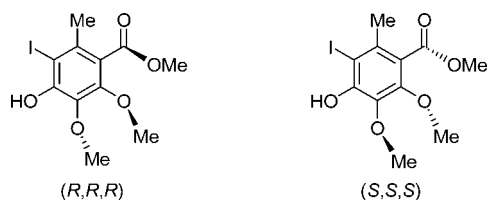
FIGURE 17. Spontaneous resolution of a calicheamicin \gamma_1^1 aromatic fragment into crystals containing enantiomers [( R,R,R ) and ( S,S,S )] (Nicolaou et al., 1988). 41
