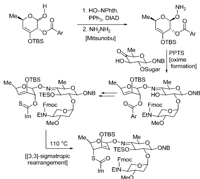
(b) Highlights of the total synthesis of calicheamicinone and calicheamicin \gamma_1^I .
