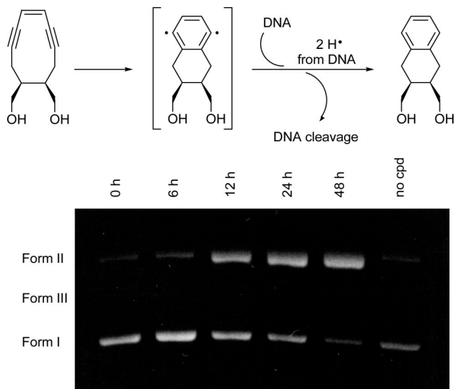
FIGURE 14. Electrophoresis gel showing \Phi X174 DNA cleavage by a designed enediyne. Forms I, II, and III refer to supercoiled, relaxed circular, and linear DNA, respectively (Nicolaou et al., 1988). 36 (Photo reprinted with permission from J. Am. Chem. Soc. , Vol. 110, p 7247. Copyright 1988 American Chemical Society.)
