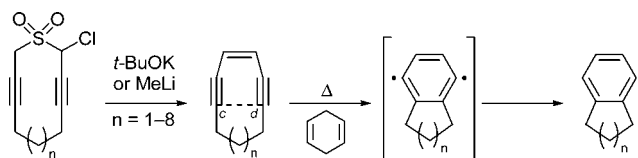
FIGURE 13. Synthesis and study of cyclic enediynes (Nicolau et al., 1988). 36
