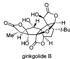
FIGURE 21. Molecular structure of ginkgolide B.
