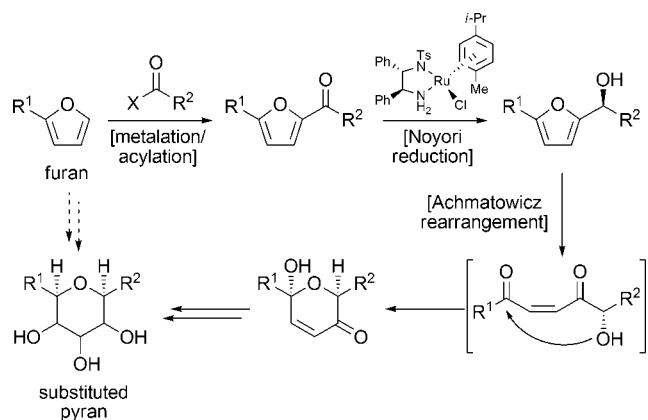
FIGURE 43. Furan-based asymmetric synthesis of substituted pyrans through a Noyori reduction and an Achmatowicz rearrangement (Nicolaou et al., 2007). 116
