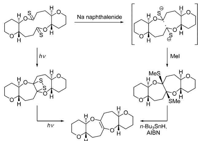
FIGURE 28. Dithionolactone bridging method of cyclic ether formation (Nicolaou et al., 1986–1988). 80,81
