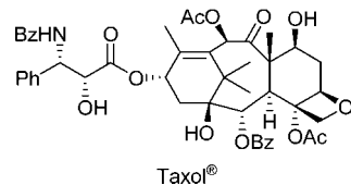
FIGURE 20. Molecular structure of Taxol.
