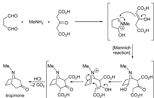
FIGURE 3. Biomimetic total synthesis of tropinone (Robinson, 1917). 8
