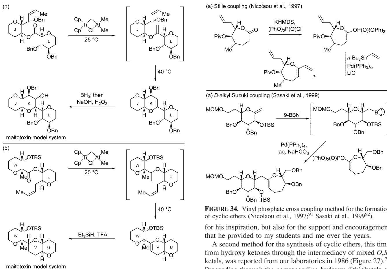
FIGURE 33. Convergent ester methylenation/metathesis approach to JKL and UVW maitotoxin model systems (Nicolaou et al., 1996). 89
