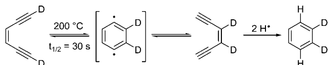
FIGURE 10. Bergman cycloaromatization reaction (Jones and Bergman, 1972). 32
