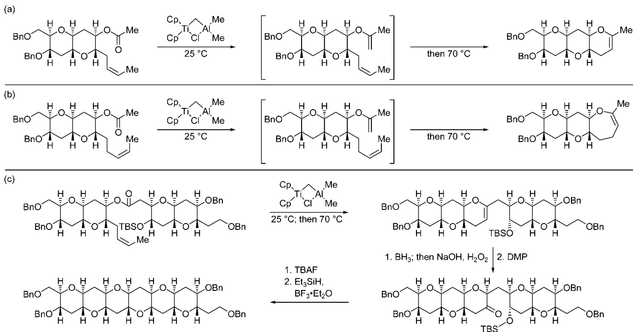
FIGURE 32. Selected examples of the one-pot titanium-mediated methylenation/ring-closing metathesis construction of complex polycyclic ethers (Nicolaou et al., 1996). 87
