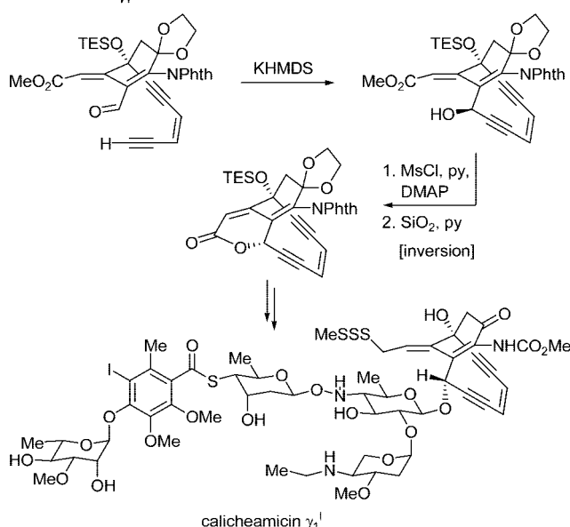
FIGURE 12. Highlights of the total synthesis of calicheamicin \gamma_1^I (Nicolau et al., 1992). 35
