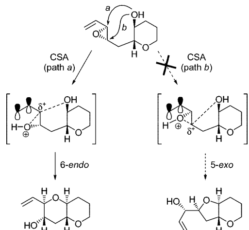
FIGURE 26. 6-Endo hydroxy epoxide opening method for cyclic ether formation (Nicolaou et al., 1985). 76
