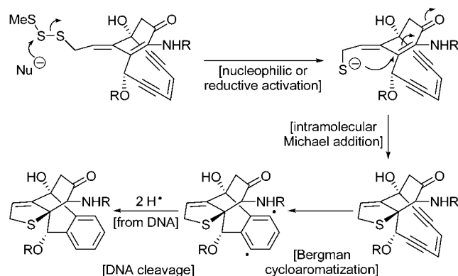
FIGURE 11. Mechanism of action of calicheamicin \gamma_1^I .
