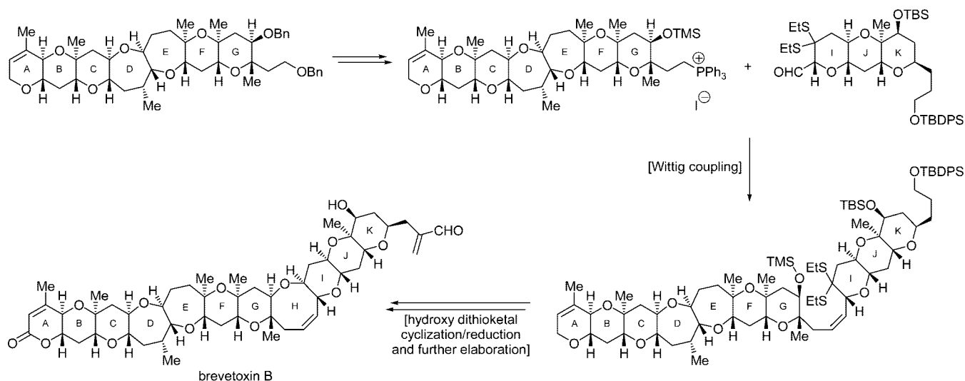
FIGURE 37. Total synthesis of brevetoxin B. Completion of the synthesis (Nicolau et al., 1995). 94
