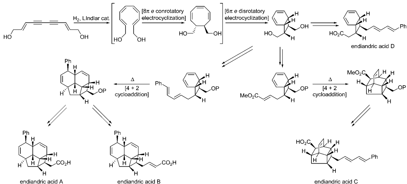
FIGURE 5. Stepwise total synthesis of endiandric acids A–D (Nicolau et al., 1982). 11
