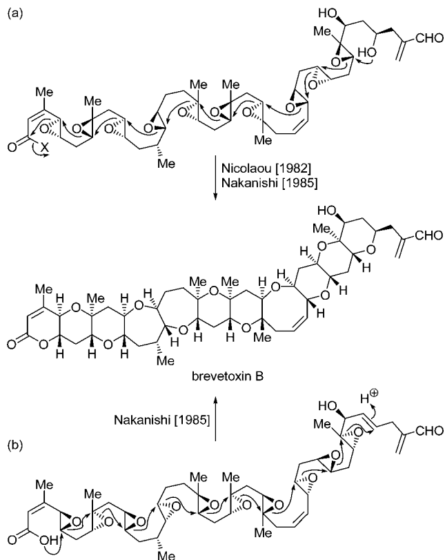
FIGURE 25. Nakanishi hypothesis for the biosynthesis of brevetoxin B [(a): Nicolaou, 1982; 73 Nakanishi, 1985; 74 (b): Nakanishi, 1985 74 ].
