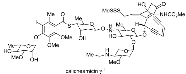
FIGURE 9. Originally proposed and revised molecular structure of calicheamicin \gamma_1^I .
