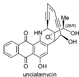
FIGURE 18. Molecular structure of uncialamycin.
