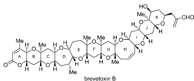
FIGURE 24. Molecular structure of brevetoxin B.
