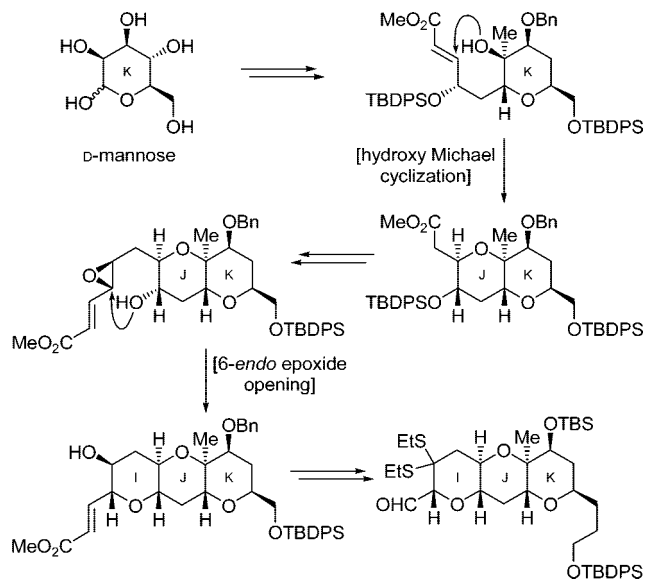
FIGURE 36. Total synthesis of brevetoxin B. Construction of the IJK domain (Nicolau et al., 1995). 94
