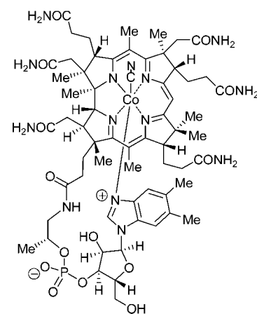
FIGURE 8. Molecular structure of vitamin B 12 .
