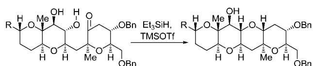
FIGURE 30. Synthesis of cyclic ethers by hydroxy ketone reductions (Nicolaou et al., 1989; 81b Evans et al., 2003; 84 Sato and Sasaki, 2007 85 ).
