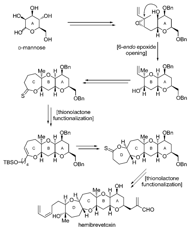
FIGURE 38. Highlights of the total synthesis of hemibrevetoxin (Nicolau et al., 1992). 95
