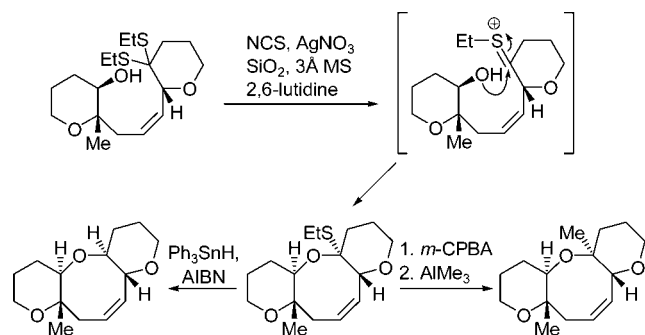
FIGURE 27. Hydroxy dithioketal cyclization method involving mixed O,S -ketals for the formation of cyclic ethers (Nicolaou et al., 1986). 79
