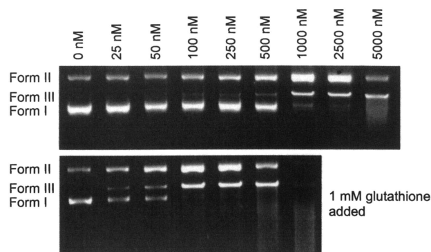
FIGURE 19. Electrophoresis gels showing single and double strand cleavage of \Phi X174 DNA by uncialamycin (Nicolaou et al., 2008). 53 (Photo: Nicolaou, K. C.; Chen, J. S.; Zhang, H.; Montero, A. Asymmetric Synthesis and Biological Properties of Uncialamycin and 26- epi -Uncialamycin. Angew. Chem., Int. Ed. 2008 , 47 , 185–189. Copyright Wiley-VCH Verlag GmbH & Co.)
