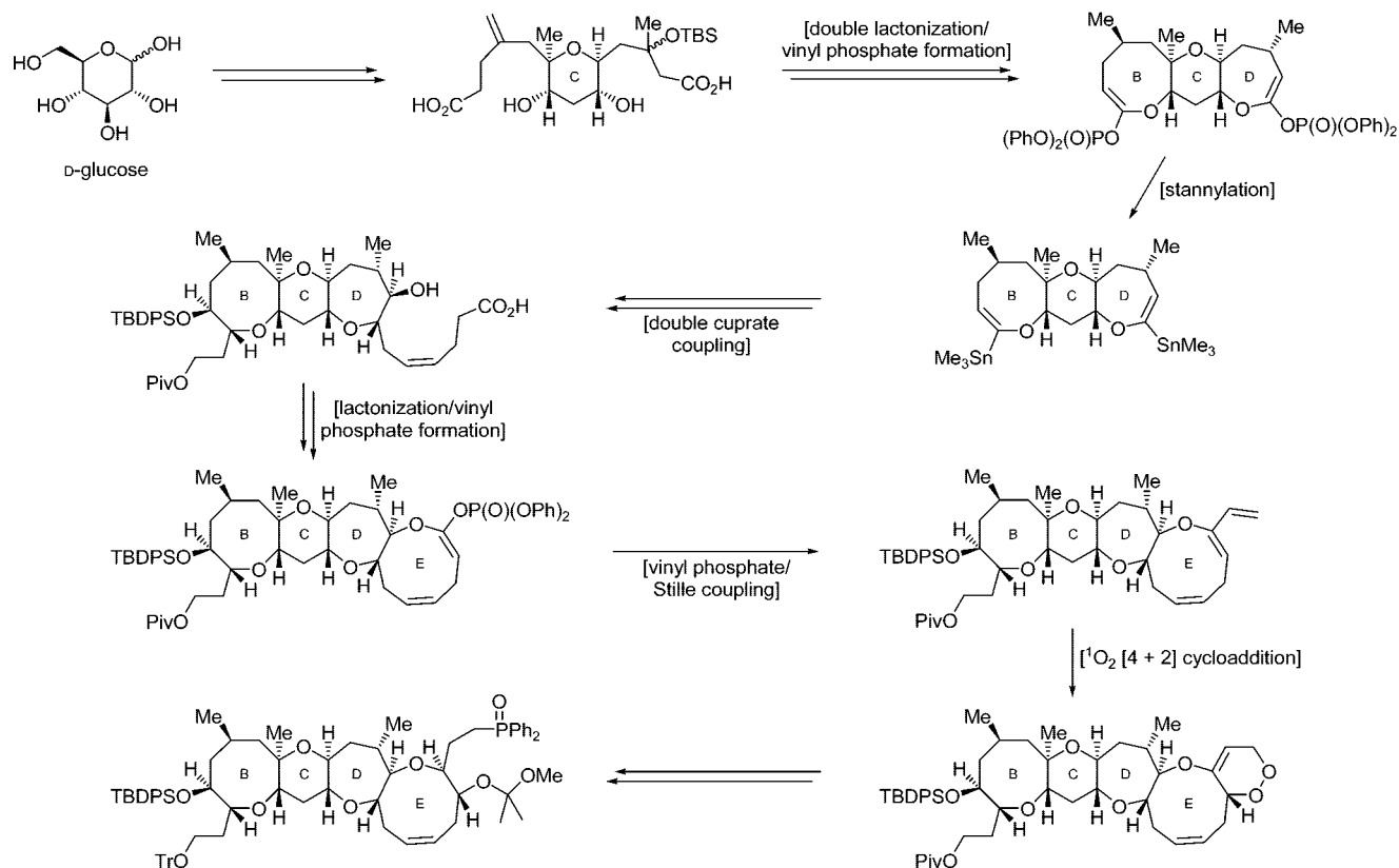
FIGURE 39. Total synthesis of brevetoxin A. Construction of the BCDE fragment (Nicolaou et al., 1998). 96
